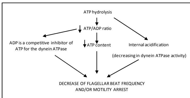
Figure 8 - ATP related facts involved in motility decrease/arrest.
