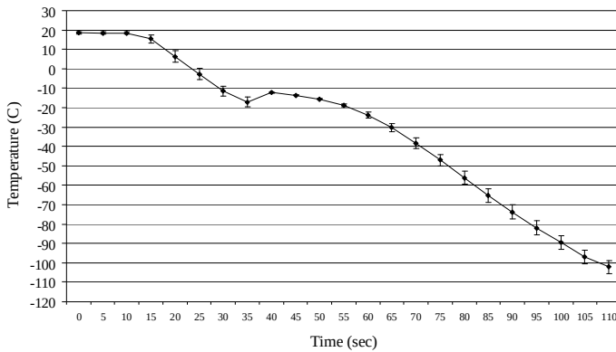
Figure 1 - Freezing curve (mean \pm SD, n = 2 ) with modified Tsvetkova's (mT) extender and 10% methanol measured in 0.5 ml French straws with a thermocouple connected to a datalogger (OM-550, Omega Engineering, Stamford, Connecticut). [5].
