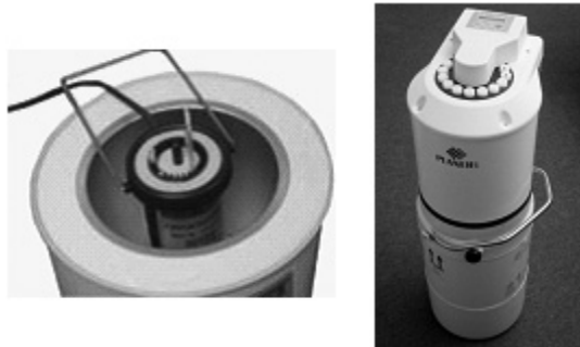
Figure 5 - Portable biofreezers: Freeze Control® (Biogenics; left) and Planer Animal Freezer® (Planer plc; right). See text for details. Source: From the respective manufacturers. With permission.
