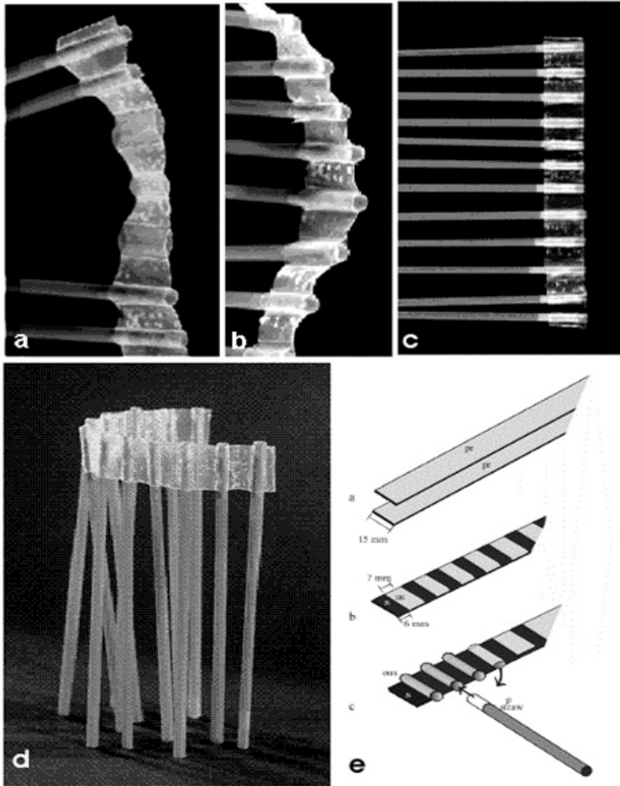
Figure 1 - Straw packages for large scale cryopreservation. (a) Plastic rack during fitting in the straws. (b) Plastic rack with straw. (c) Straw package, placed horizontally as done for freezing. (d) Straw package rolled together as done for storage and for cutting open. (e) Steps in the production of flexible plastic racks: 1) plastic ribbons are placed one above each other, 2) plastic ribbons are sealed together, 3) the unsealed portions are opened and straws are fitted in. (Source: Lahnsteiner F., N. Mansour and T. Weismann, Aquaculture 209: 359-367, 2002. With permission).
