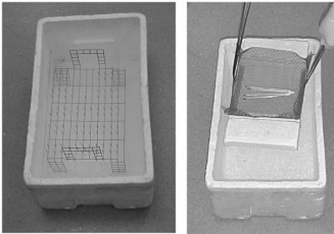
Figure.1 - \text{LN}_2 vapour freezing method: styrofoam box with home-made straw holder for placing samples above \text{LN}_2 surface (left) and floating device made of styrofoam and plastic net (right). (Source: E. Cabrita.)
