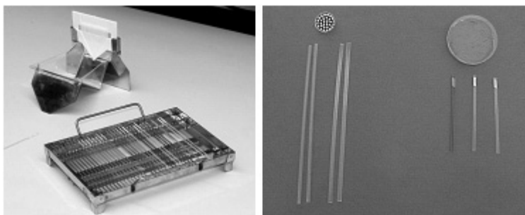
Figure 11 - Left: 0.25-mL straws on a metallic straw holder ready to be cryopreserved; next to the holder there is a boat with a plastic comb, used to remove excess sample from the straws which enables sealing of the open end. Right: comparison between macrotubes (2 mL) and straws (0.25 mL); two sealing materials are shown: metallic balls for the macrotubes and polyvinyl powder for the straws. Source: Dr. F. Martínez-Pastor and Dr. E. Cabrita. With permission.
