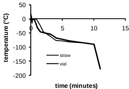
Figure 1 - Record of temperature decrease during the process.
