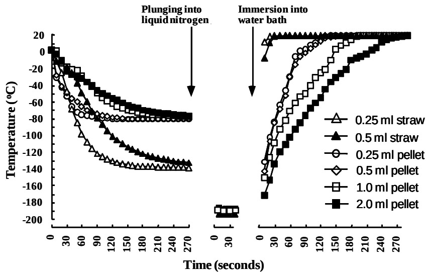
Figure 1 - Temperature during cooling of diluted semen (initially at 2°C, semen diluted 1:5, semen: DMSO diluent) in the centre of straws on styrofoam rafts in the vapour 4 cm above liquid nitrogen and in the centre of pellets on dry ice, after plunging into liquid nitrogen and after immersion (straws transferred directly, pellets in dry test tubes) into a waterbath at 20°C. Adapted from Ritar and Campet [8].
