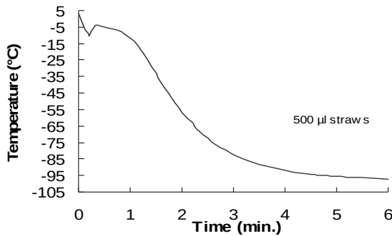
Figure 2 - Temperature decrease in 0.5 ml French straws laid 3 cm above liquid nitrogen. Crystallization occurs at -10^{\circ}\text{C} . No seeding is required.
