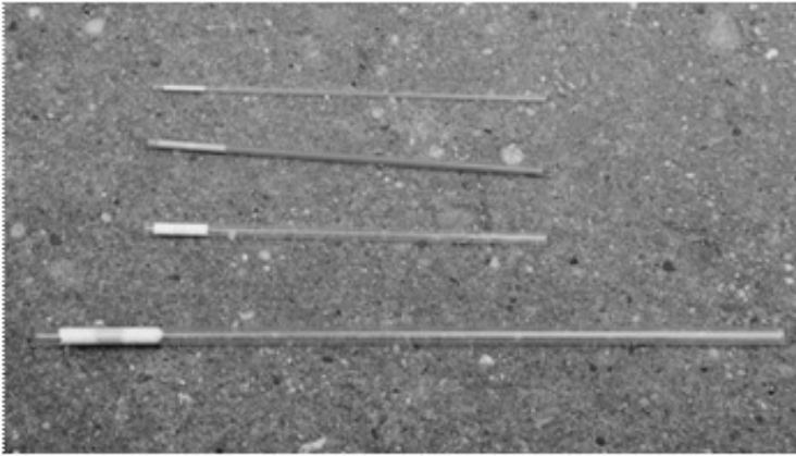
Figure 2 - Different straw types used for the cryopreservation of fish sperm (from top to bottom): 0.25 ml straw, 0.5 ml straw, 1.2 ml straw and 4 ml straw with a home-made cotton plug.
