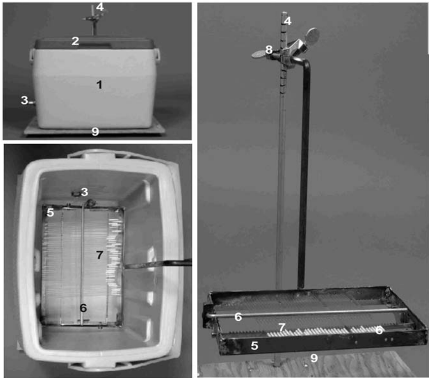
Figure 3 - (top left) Freezing apparatus built out of a commercial freezing box. (bottom left) Open-freezing box showing the freezing rack loaded with 0.5 ml straws. (right) Commercial available freezing rack originally used for freezing of bull semen and loaded with 0.5 ml straws. Rack can be moved up and down on a marked scale. 1: freezing box; 2: cover of the freezing box; 3: liquid nitrogen drainage tap; 4: marked scale; 5: freezing rack; 6: metal bar to prevent the straws from floating when plunging into the liquid nitrogen; 7: 0.5 ml straws; 8: screw clamp for changing the level of the freezing rack above the surface of liquid nitrogen; 9: wooden base. The freezing box has the following dimensions: Inner length: 34 cm, inner width: 31 cm, inner height: 22 cm, drainage hole of liquid nitrogen: 7 cm above bottom, wall thickness: 3 cm.
