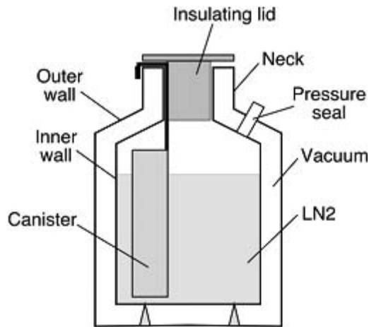
Figure 6 - Schematic diagram of a general LN_2 Dewar. Note the insulating structure formed by a double wall enclosing a vacuum.
