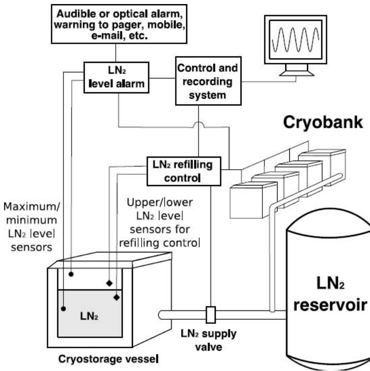
Figure 8 - Scheme of a large cryobank provided with refilling and control facilities.
