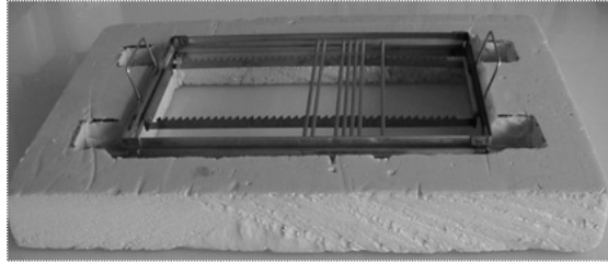
Figure 1 - Freezing rack and the polystyrene frame
