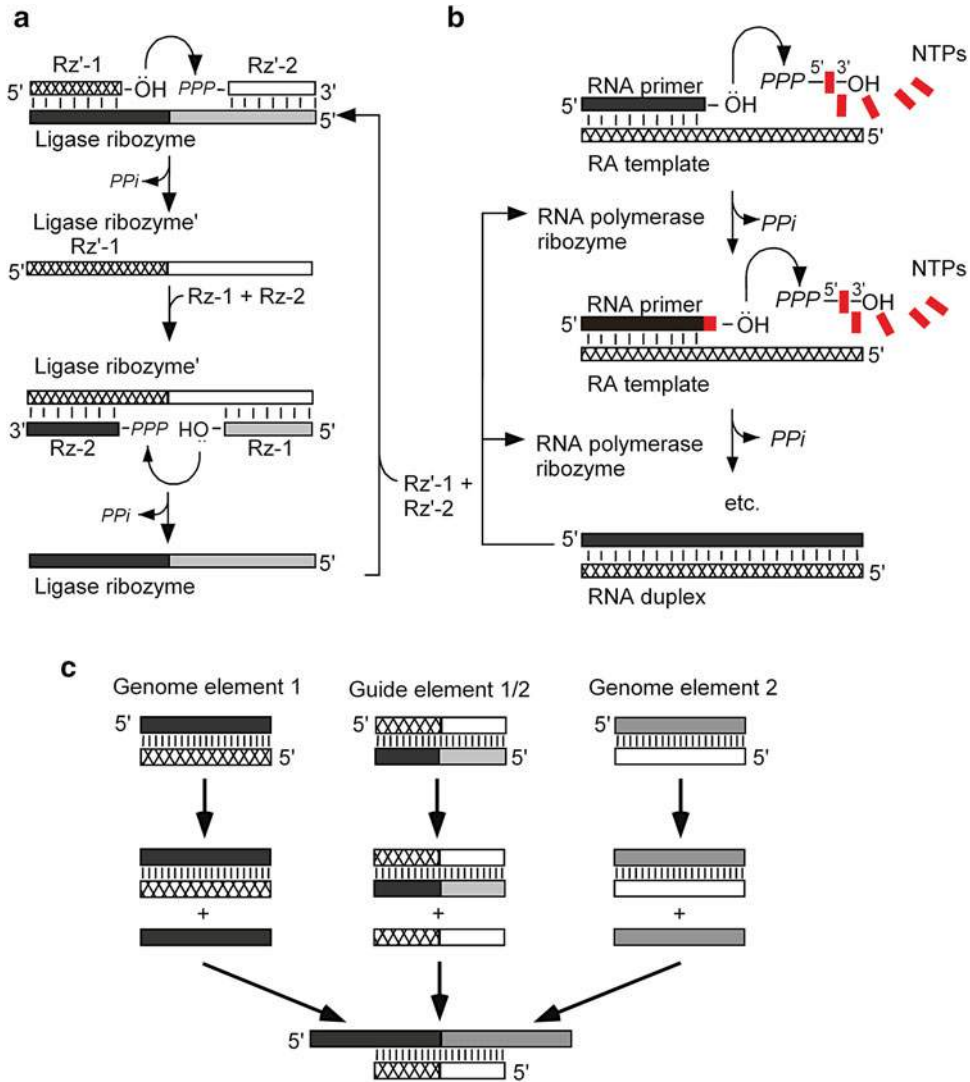
Fig. 7.1 Model of the putative primordial replicator. (a) Cross-replication of RNA ligase ribozymes: a ligase ribozyme (gray and black) catalyzes the ligation of white and crossed oligonucleotides ( Rz'-1 and Rz'-2 ) to generate a ligase ribozyme that catalyzes the ligation of black and gray oligonucleotides ( Rz-1 and Rz-2 ) to regenerate the first ligase ribozyme. (b) Ribozyme-catalyzed RNA polymerization. The complete extension of an RNA primer (black) according to the sequence of a template
